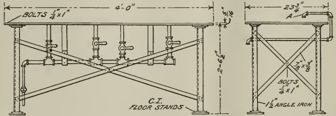
BENCH FOR AIR TEMPERING OF TOOLS.
